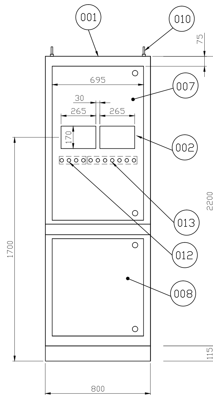
INTERNAL FRONT VIEW (WITH INNER DOOR)
