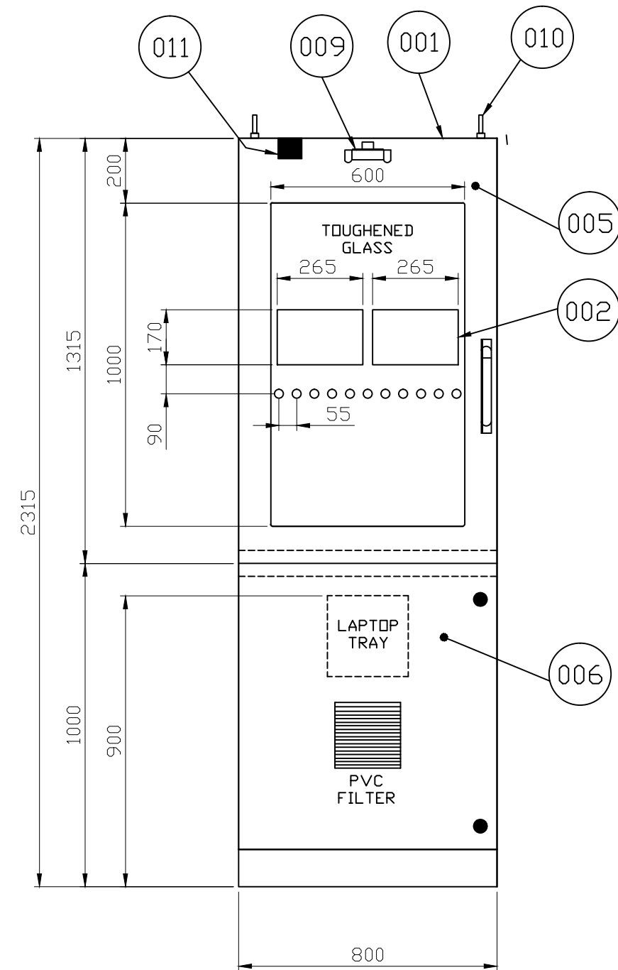
FRONT VIEW
