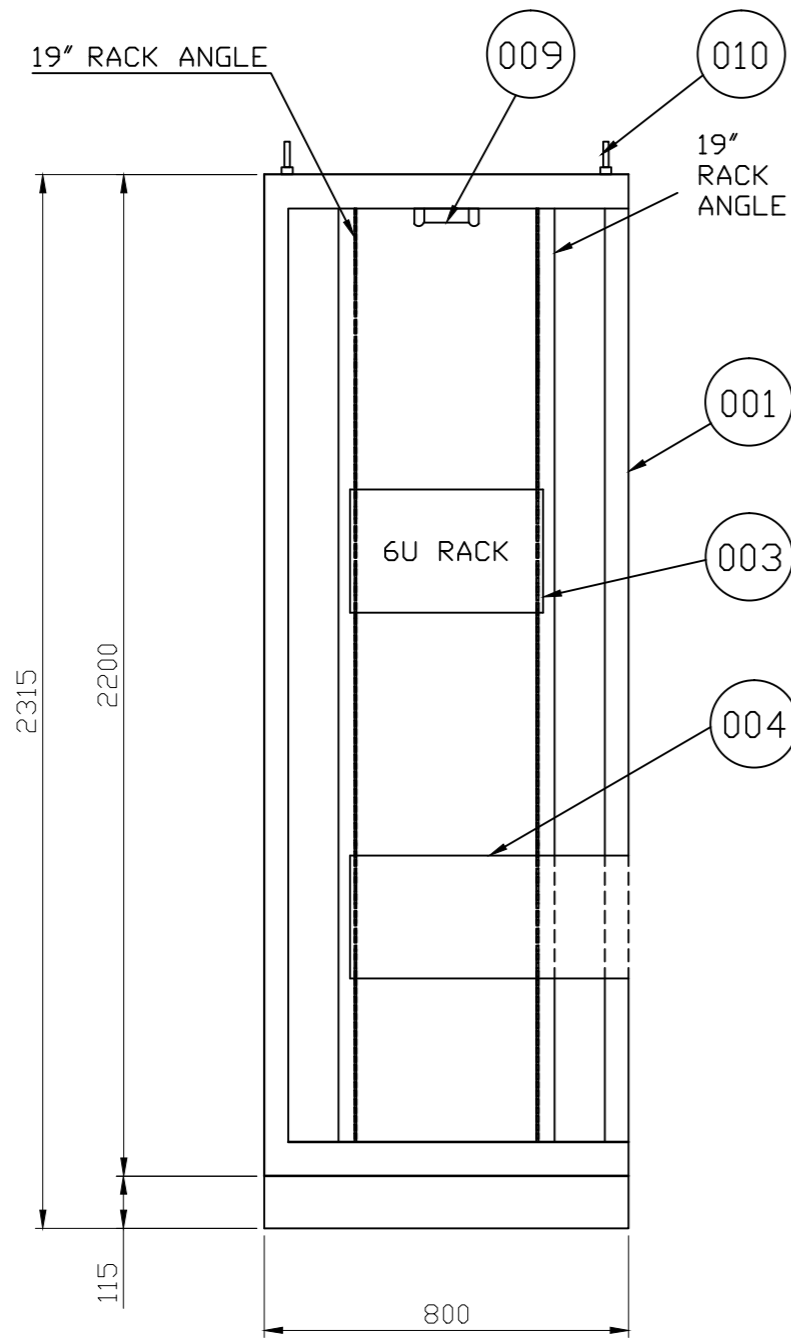
INTERNAL FRONT VIEW WITHOUT INTERNAL DOOR
