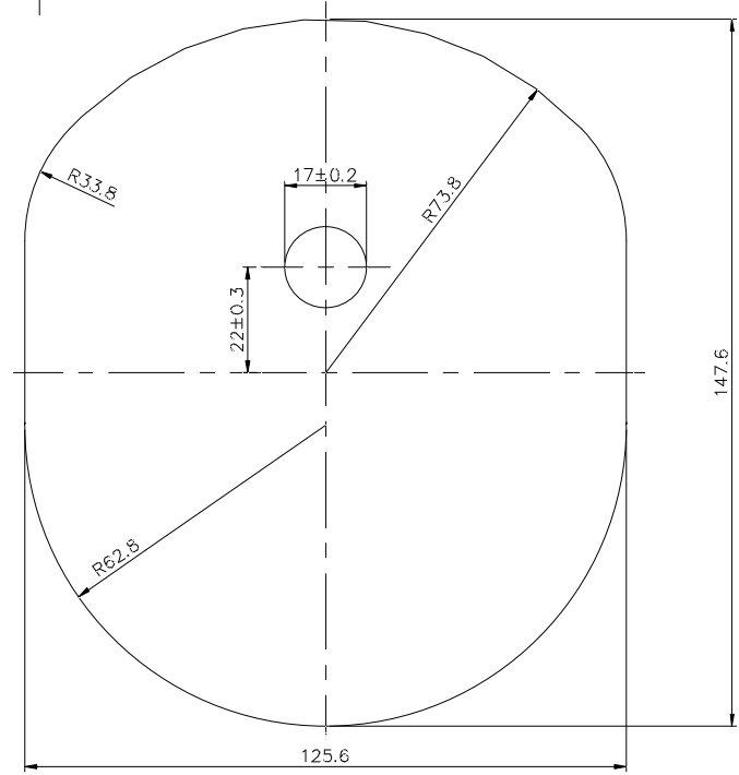
DEVELOPED VIEW OF IT.001
