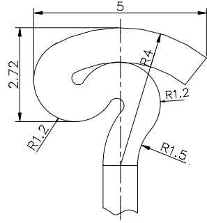
DETAIL-X (SCALE-10:1)
