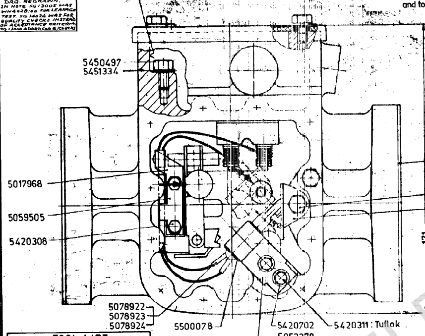
TOP VIEW WITHOUT COVERING & COVER
