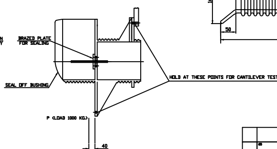
DETAIL-Y
