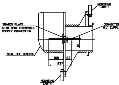
DETAIL-X
