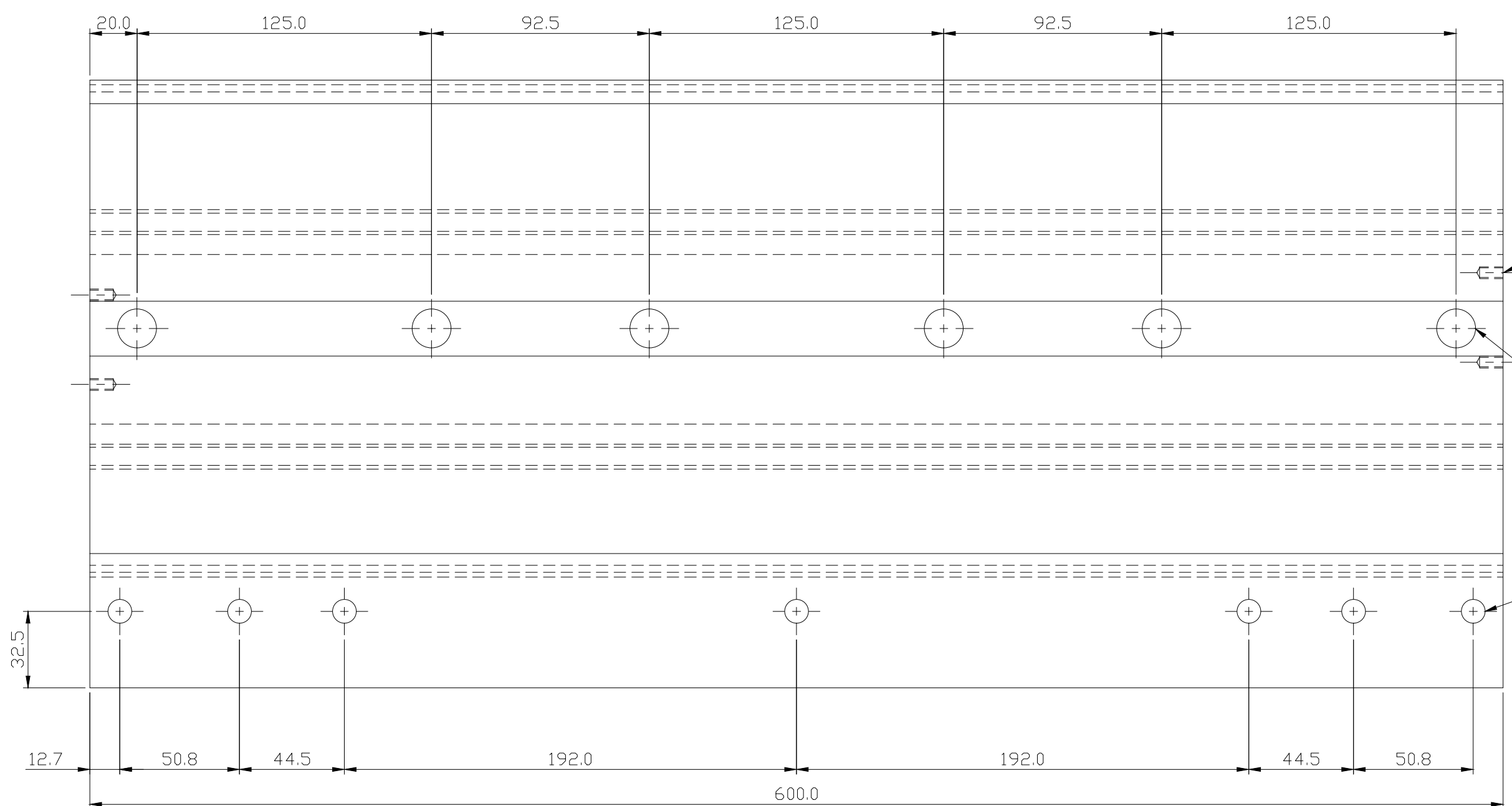
PLAN
