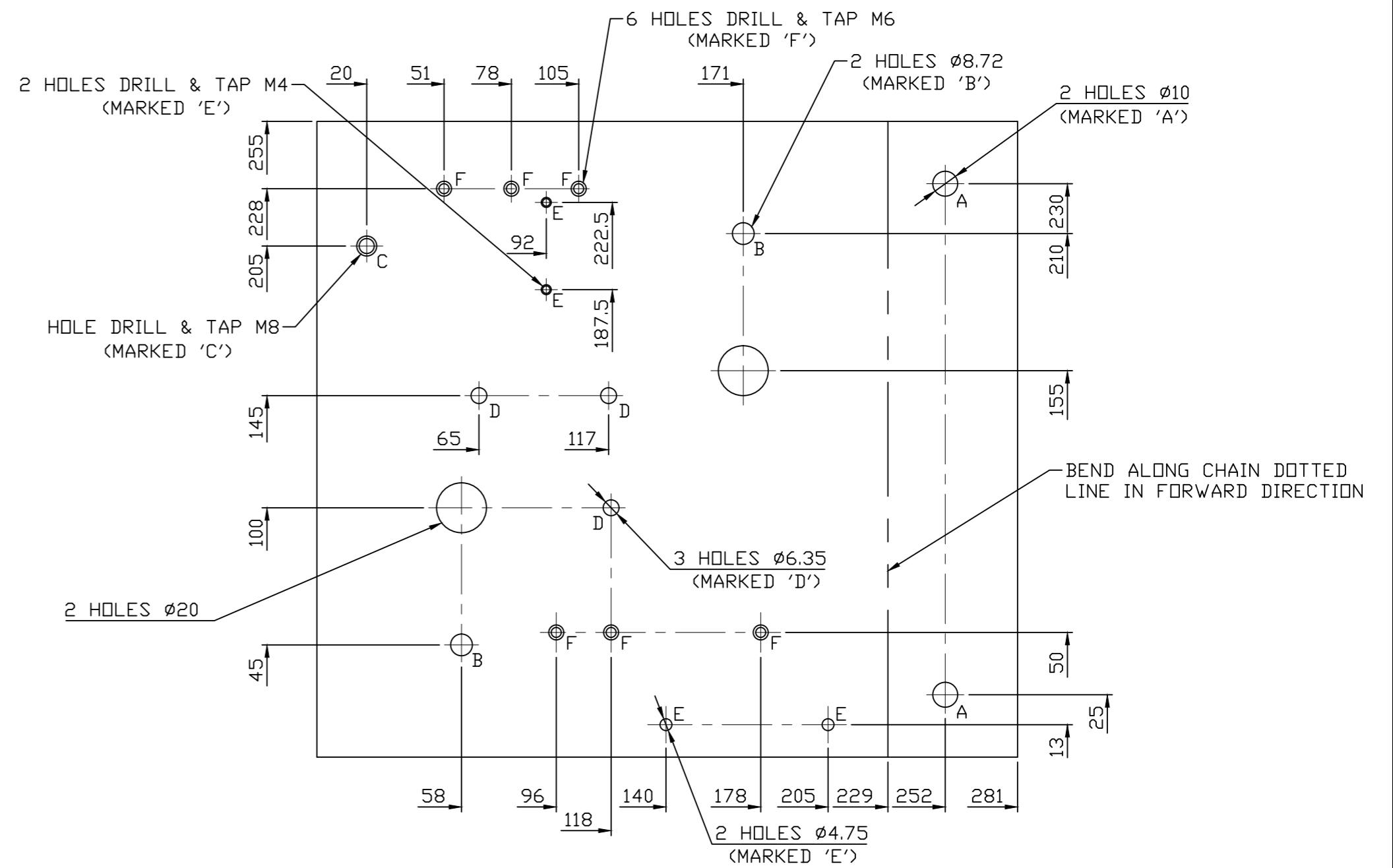
DEVELOPED VIEW OF IT. 001
