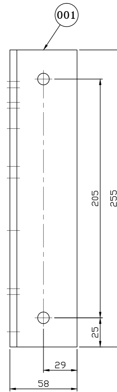
SIDE VIEW
