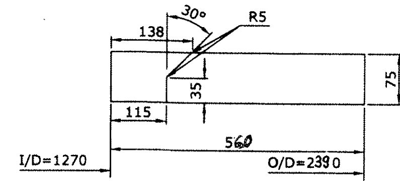
SECTION B-B SEE NOTE-1
