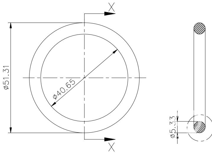
SECTION-XX
