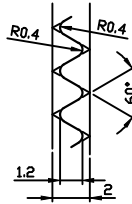
TOOTH PROFILE AT \phi 56 (SCALE 5:1)
