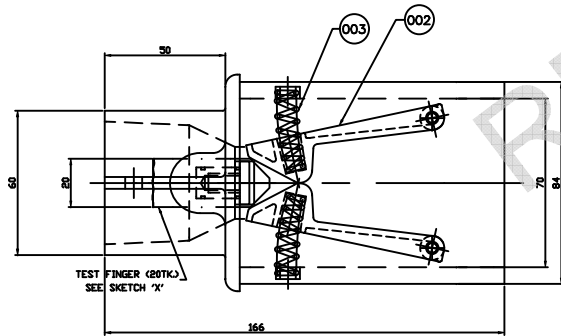
SHUTTER CLOSED POSITION
