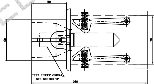
SHUTTER OPEN POSITION
